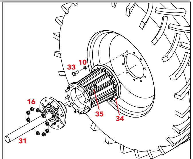
VIEW A
