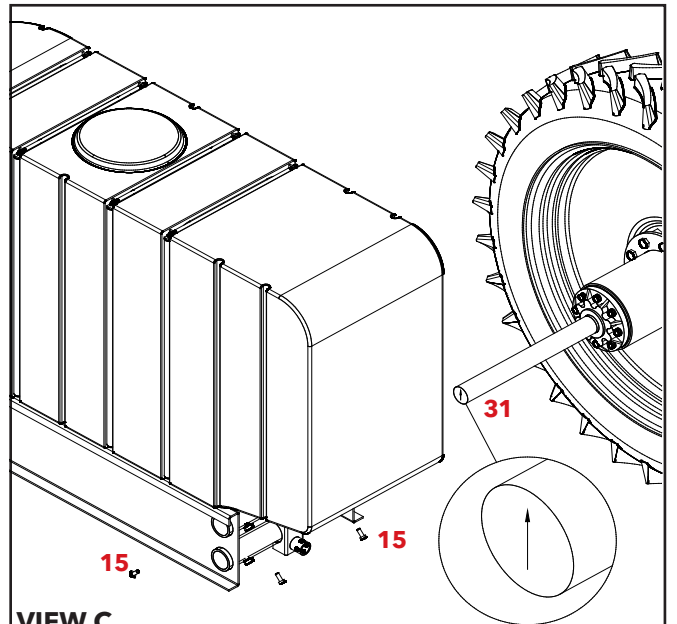
VIEW C
